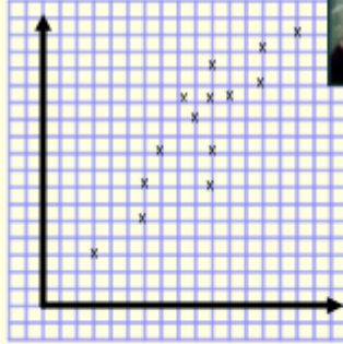
Positive Correlation
