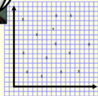
No Correlation
